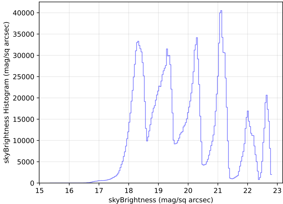
too_elab_heavy_r128_d2_griz_v3.4_10yrs WFD all bands: skyBrightness Histogram
