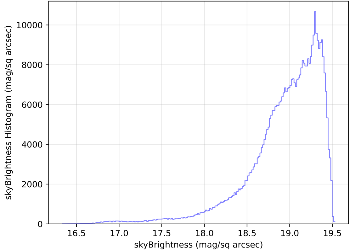
too_elab_heavy_r128_d2_griz_v3.4_10yrs All sky z band: skyBrightness Histogram
