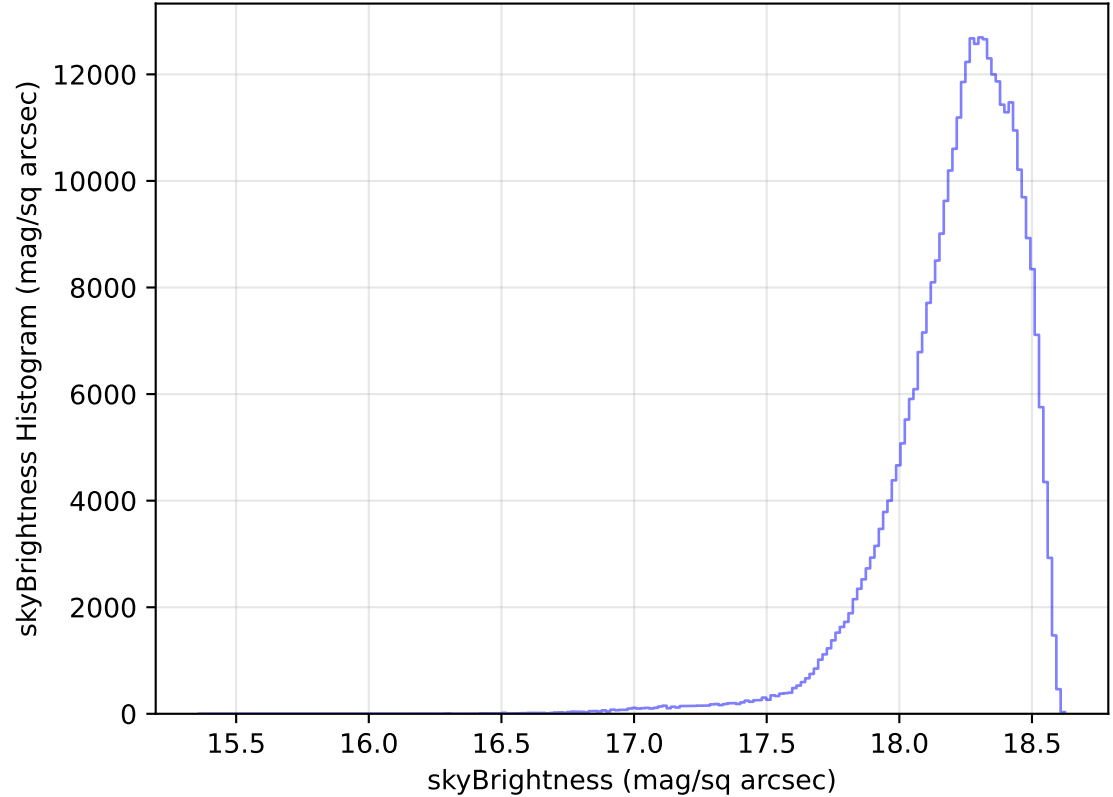
too_elab_heavy_r128_d2_griz_v3.4_10yrs All sky y band: skyBrightness Histogram
