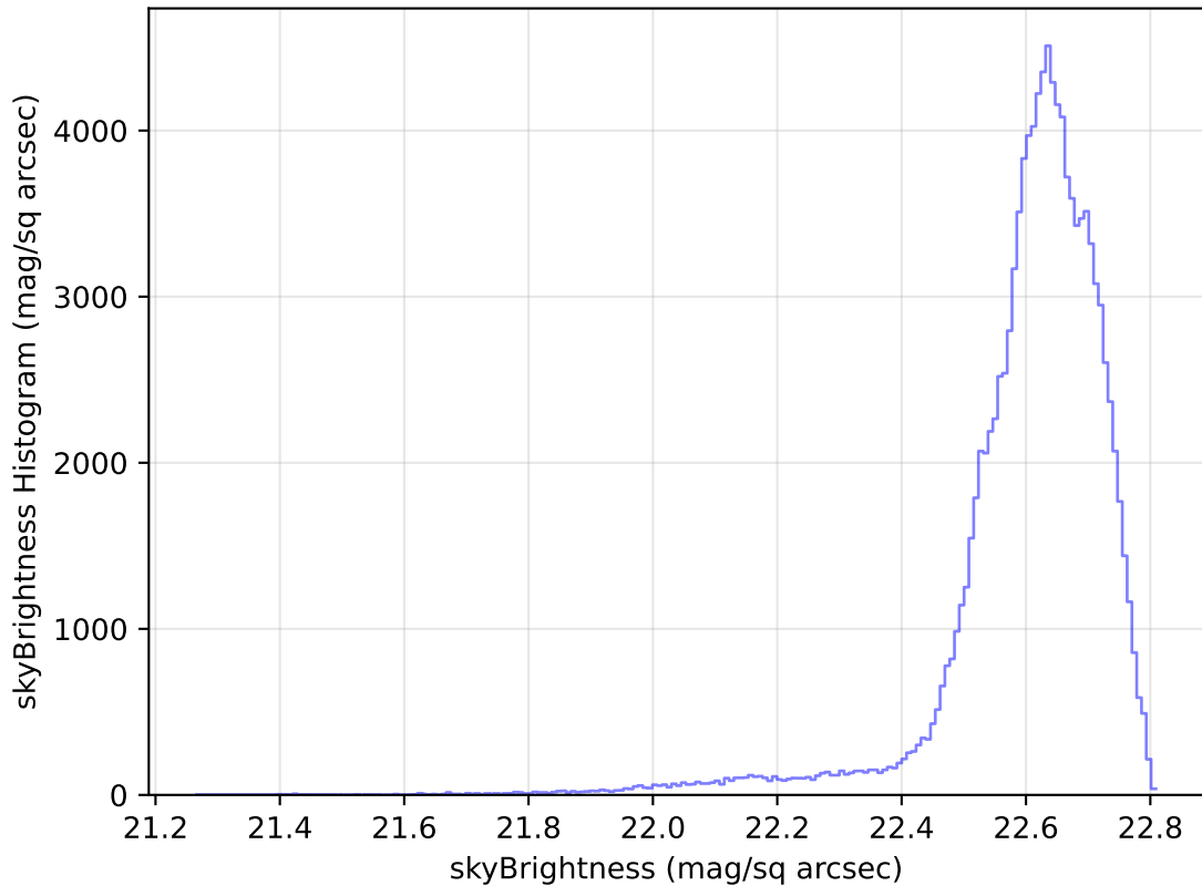
too_elab_heavy_r128_d2_griz_v3.4_10yrs All sky u band: skyBrightness Histogram
