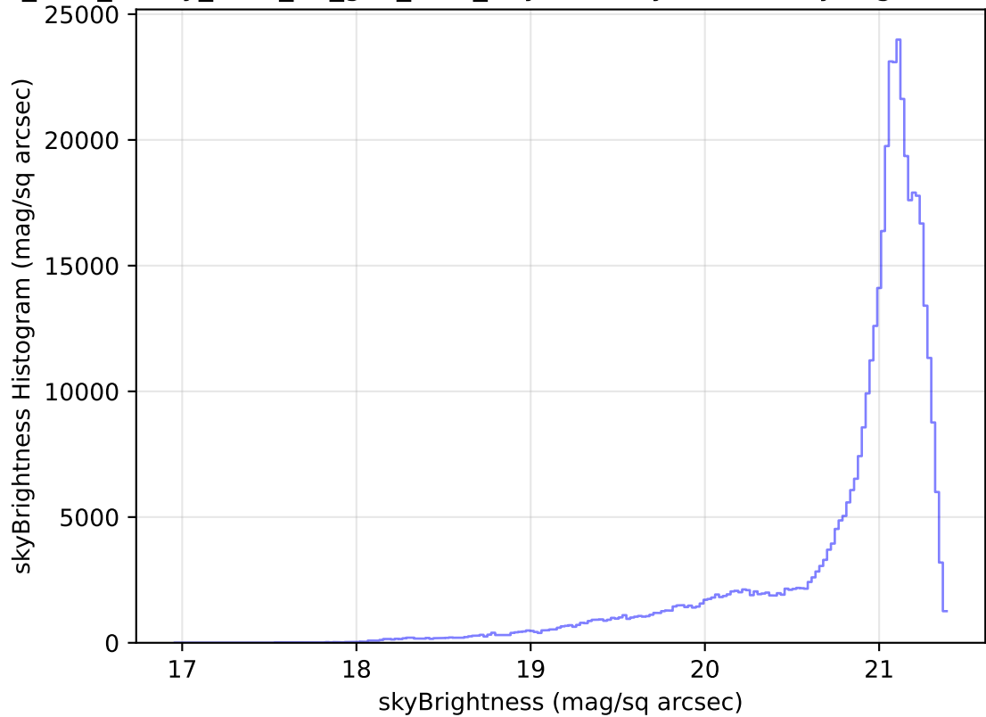
too_elab_heavy_r128_d2_griz_v3.4_10yrs All sky r band: skyBrightness Histogram
