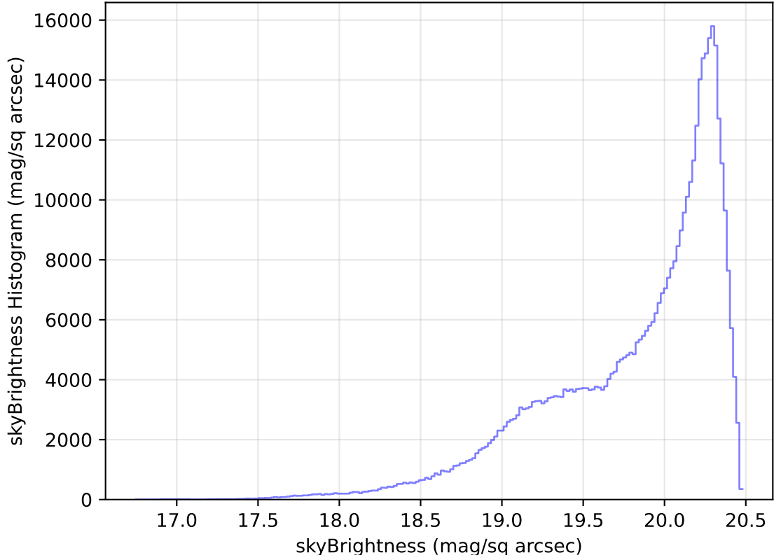
too_elab_heavy_r128_d2_griz_v3.4_10yrs All sky i band: skyBrightness Histogram
