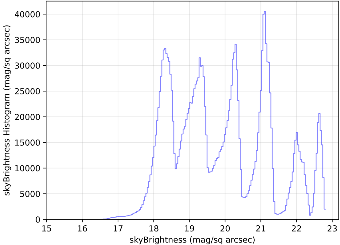
too_elab_heavy_r128_d2_griz_v3.4_10yrs All sky all bands: skyBrightness Histogram
