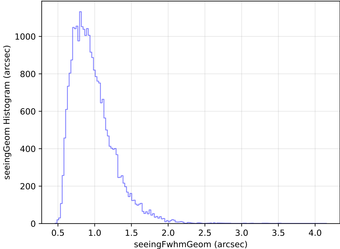
too_elab_heavy_r128_d2_griz_v3.4_10yrs Yr 1 g band: seeingGeom Histogram
