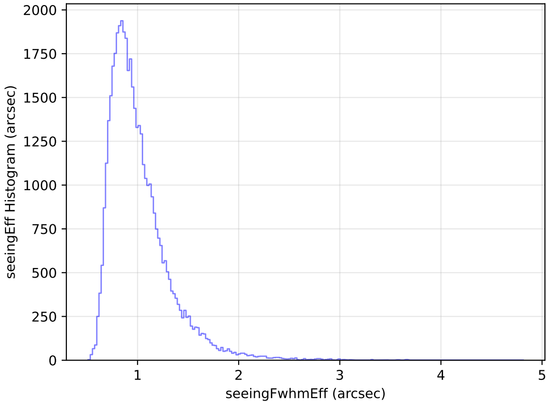
too_elab_heavy_r128_d2_griz_v3.4_10yrs Yr 1 z band: seeingEff Histogram
