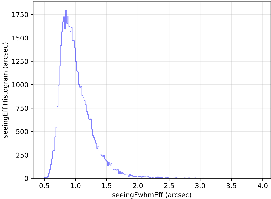
too_elab_heavy_r128_d2_griz_v3.4_10yrs Yr 1 y band: seeingEff Histogram
