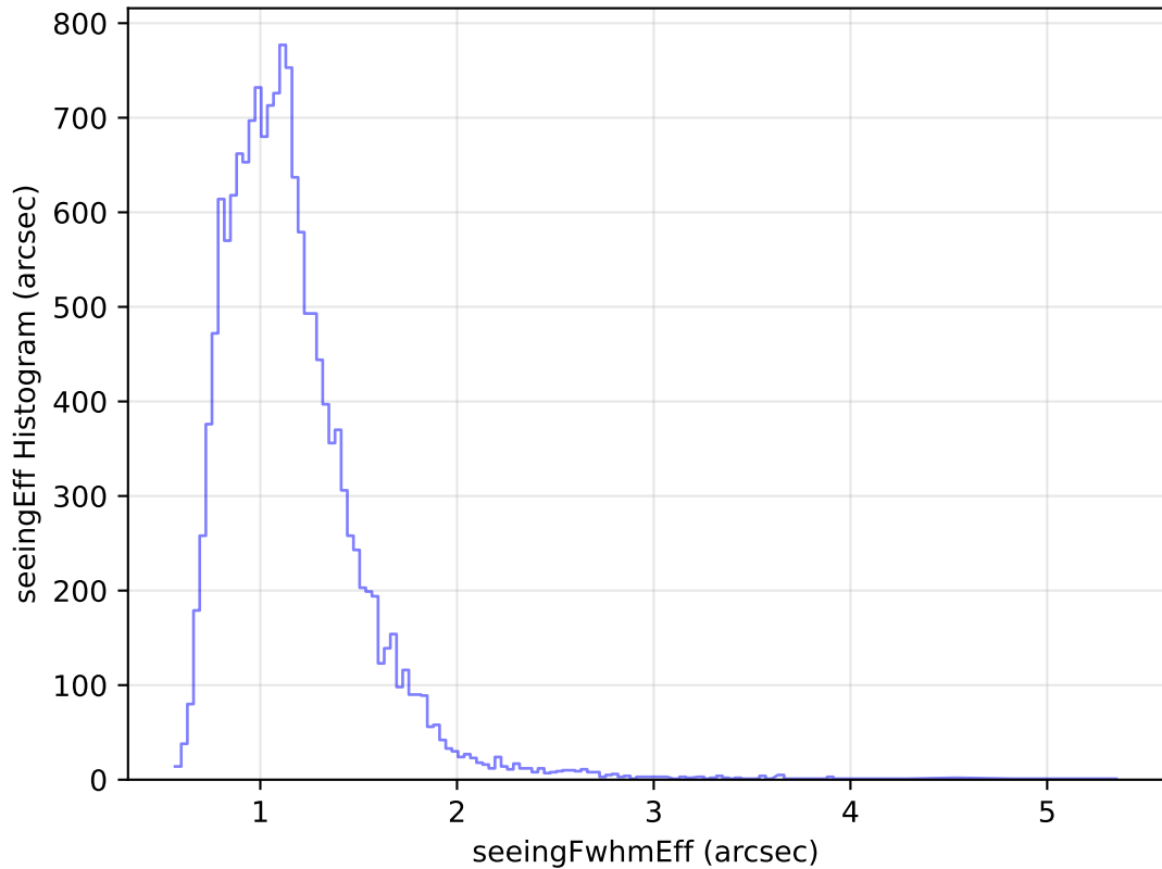
too_elab_heavy_r128_d2_griz_v3.4_10yrs Yr 1 u band: seeingEff Histogram
