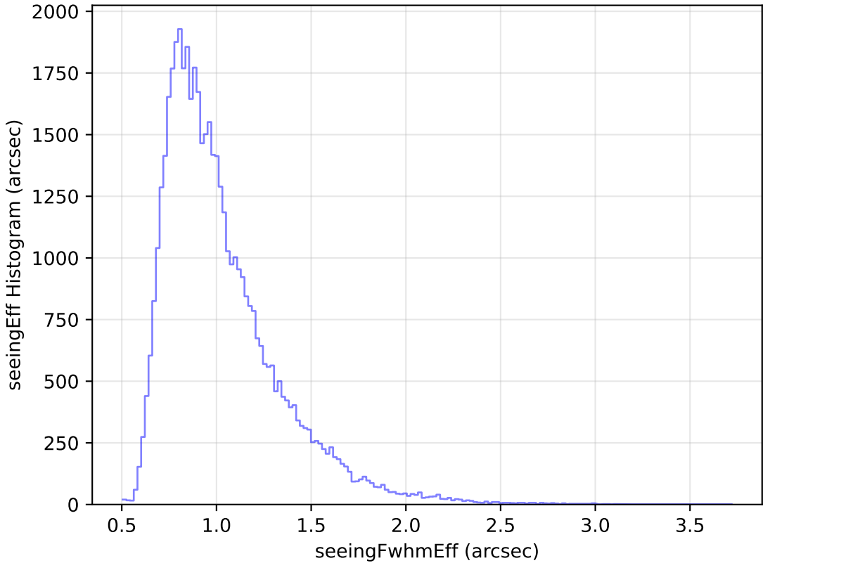
too_elab_heavy_r128_d2_griz_v3.4_10yrs Yr 1 r band: seeingEff Histogram
