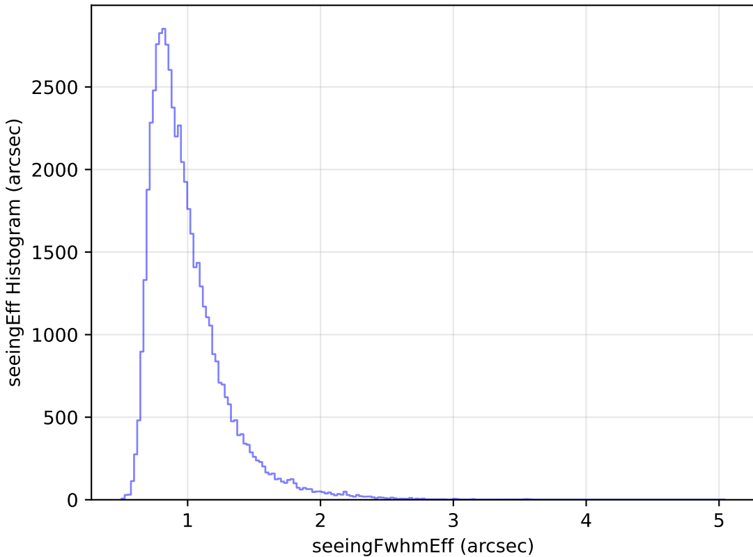
too_elab_heavy_r128_d2_griz_v3.4_10yrs Yr 1 i band: seeingEff Histogram
