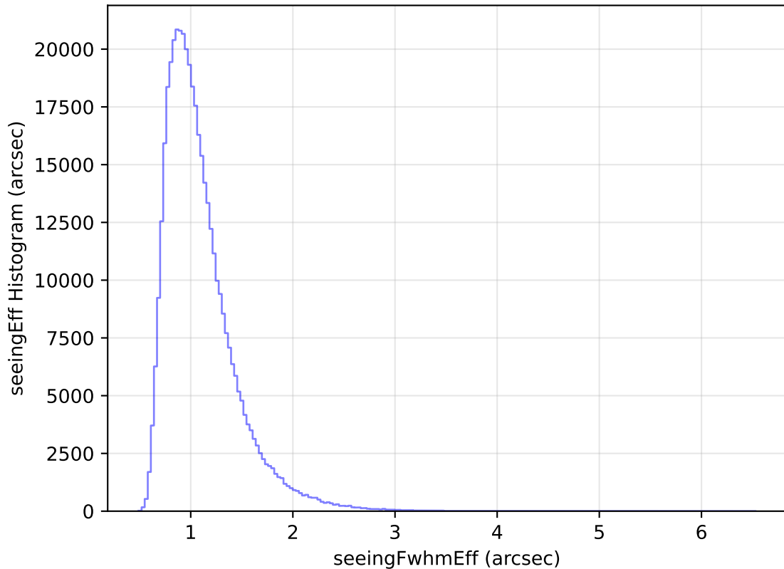
too_elab_heavy_r128_d2_griz_v3.4_10yrs WFD z band: seeingEff Histogram
