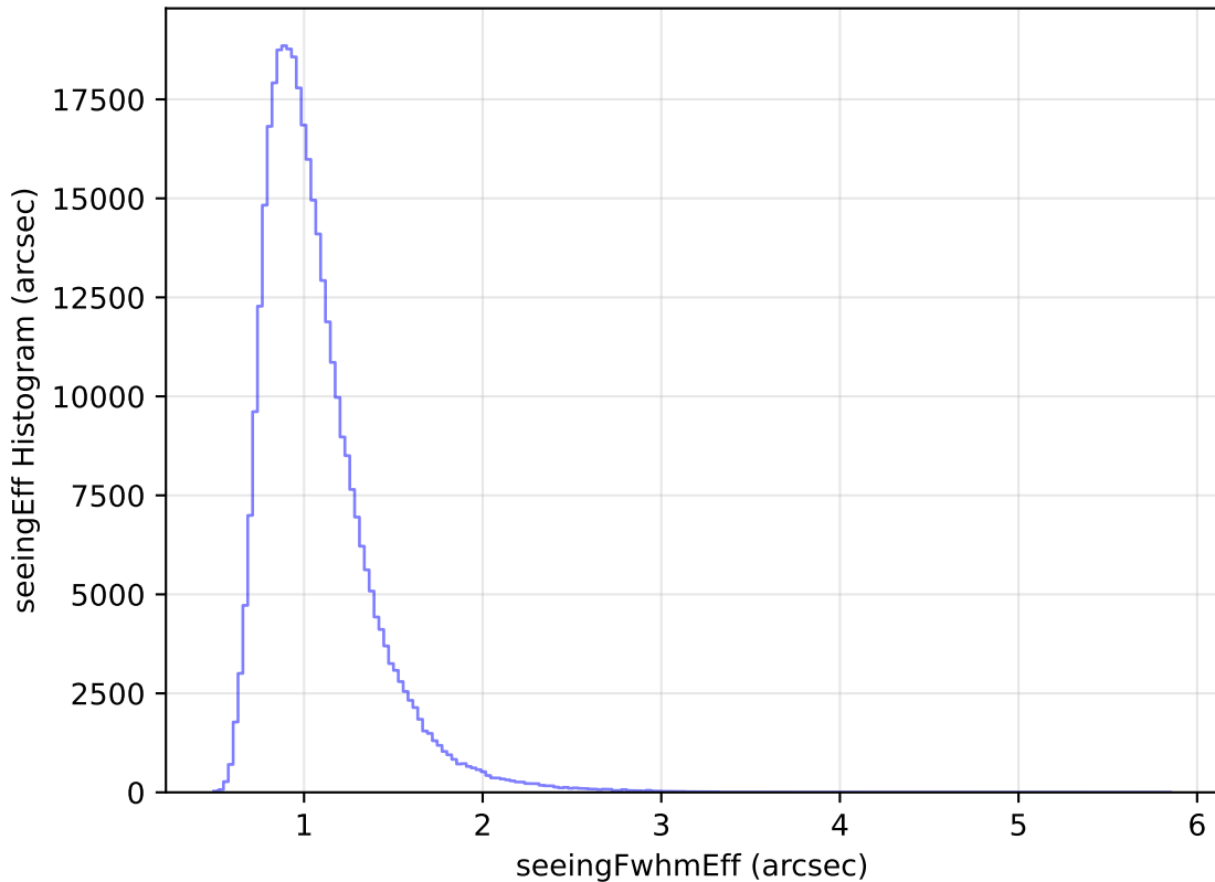
too_elab_heavy_r128_d2_griz_v3.4_10yrs WFD y band: seeingEff Histogram
