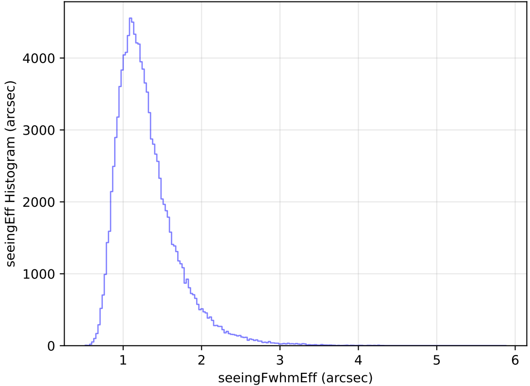
too_elab_heavy_r128_d2_griz_v3.4_10yrs WFD u band: seeingEff Histogram
