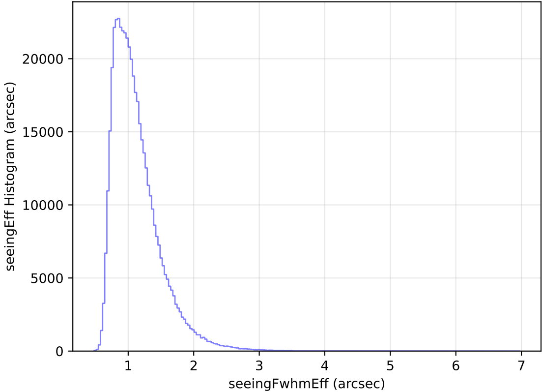
too_elab_heavy_r128_d2_griz_v3.4_10yrs WFD r band: seeingEff Histogram
