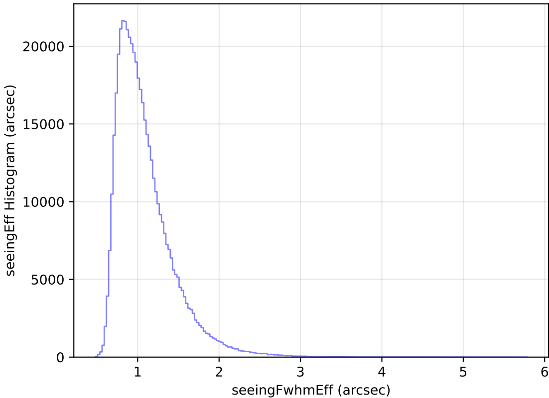
too_elab_heavy_r128_d2_griz_v3.4_10yrs WFD i band: seeingEff Histogram
