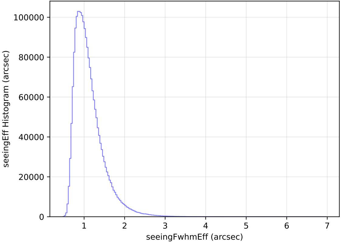
too_elab_heavy_r128_d2_griz_v3.4_10yrs WFD all bands: seeingEff Histogram
