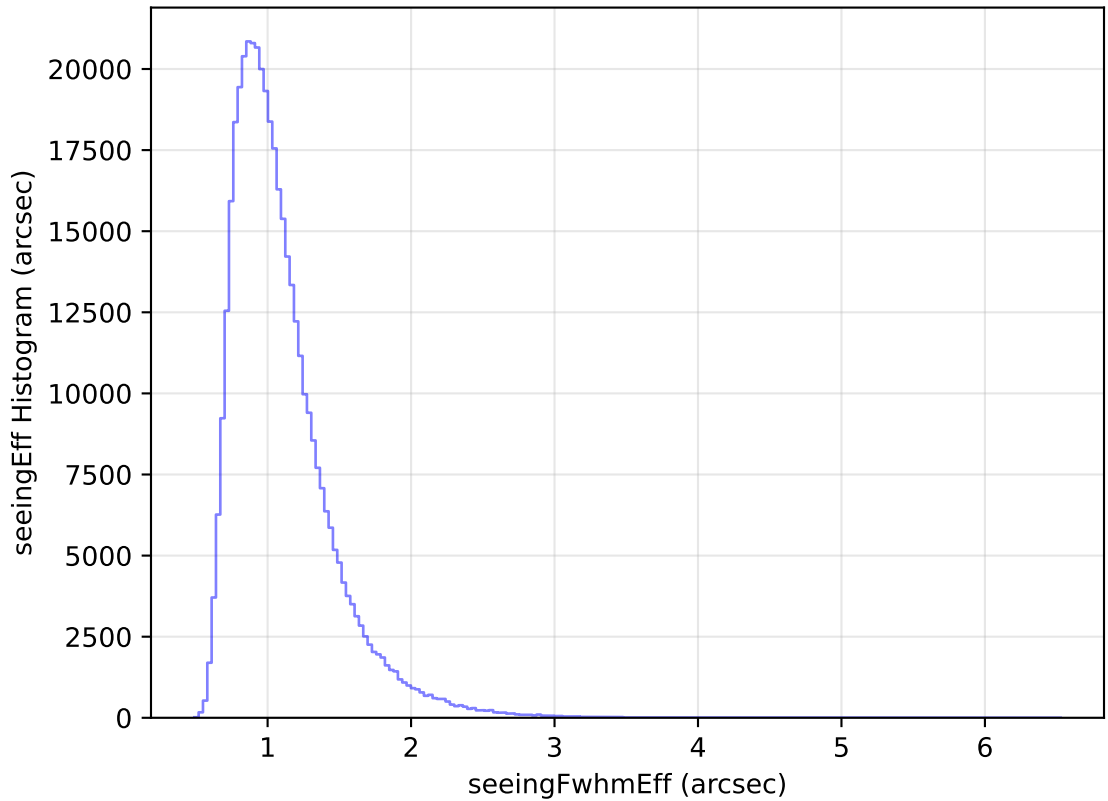
too_elab_heavy_r128_d2_griz_v3.4_10yrs All sky z band: seeingEff Histogram
