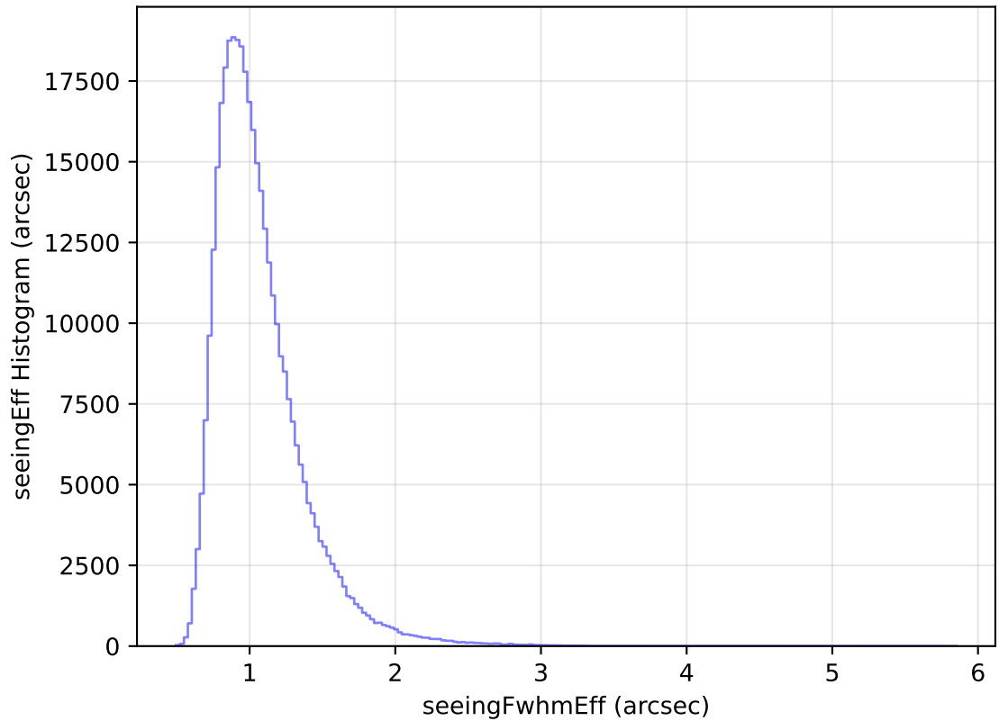
too_elab_heavy_r128_d2_griz_v3.4_10yrs All sky y band: seeingEff Histogram
