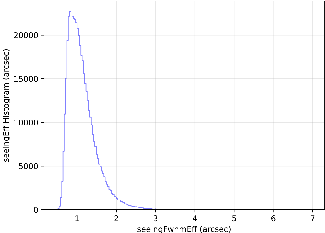
too_elab_heavy_r128_d2_griz_v3.4_10yrs All sky r band: seeingEff Histogram
