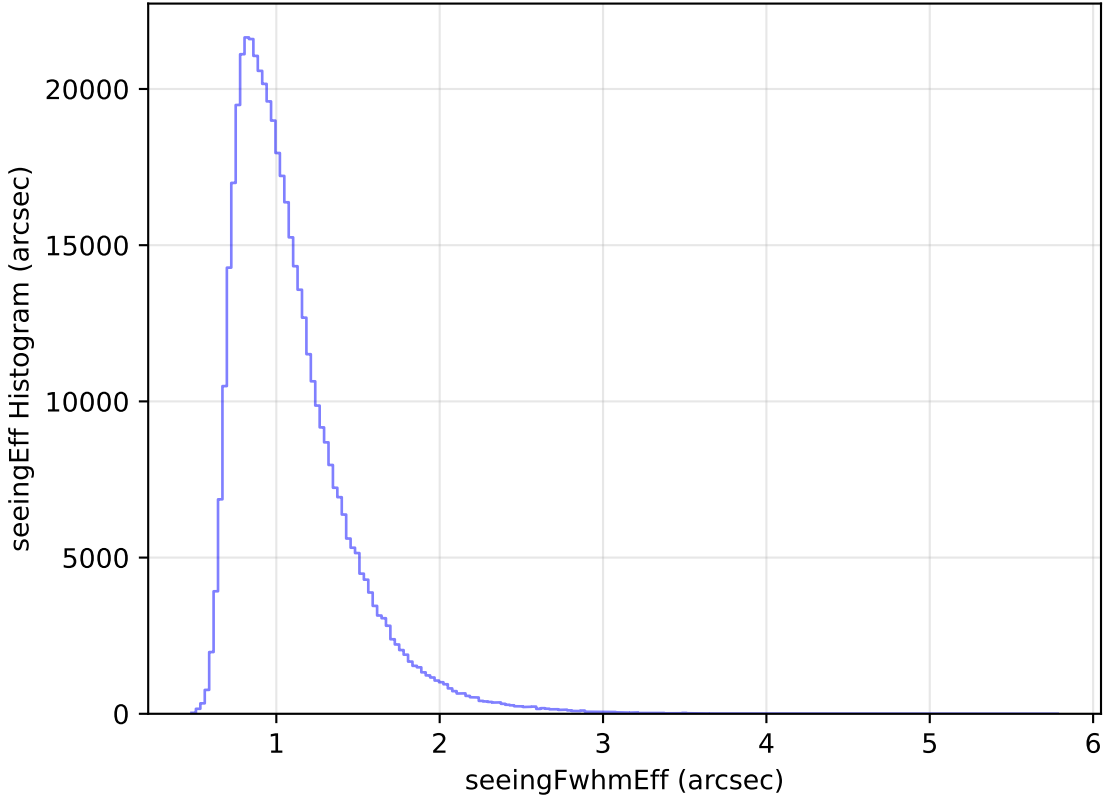
too_elab_heavy_r128_d2_griz_v3.4_10yrs All sky i band: seeingEff Histogram
