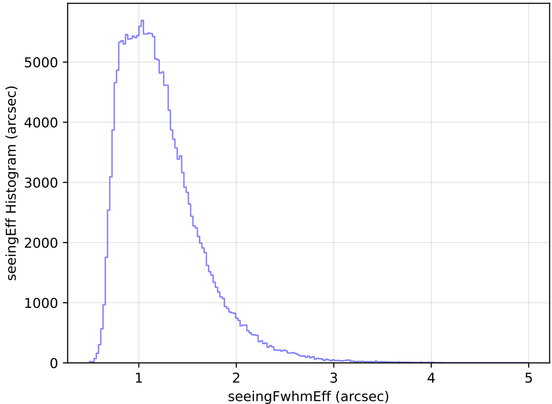
too_elab_heavy_r128_d2_griz_v3.4_10yrs All sky g band: seeingEff Histogram
