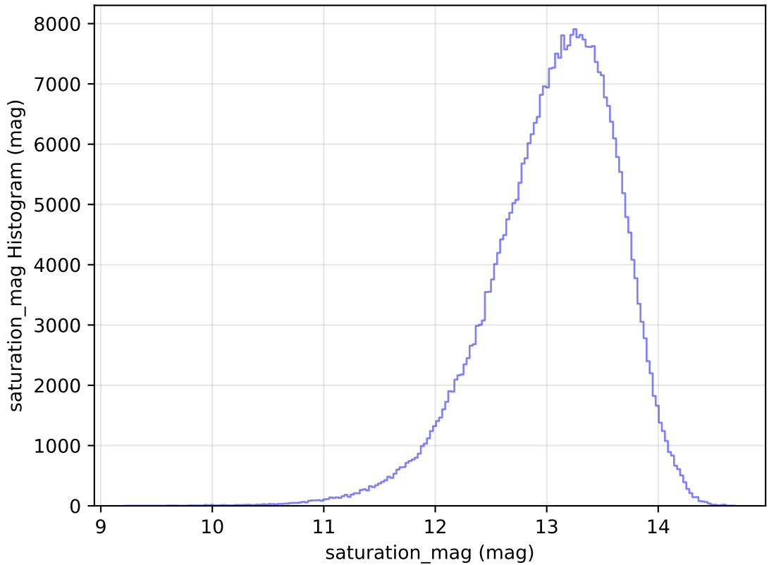
too_elab_heavy_r128_d2_griz_v3.4_10yrs WFD y band: saturation_mag Histogram
