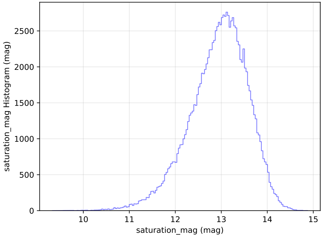
too_elab_heavy_r128_d2_griz_v3.4_10yrs WFD u band: saturation_mag Histogram
