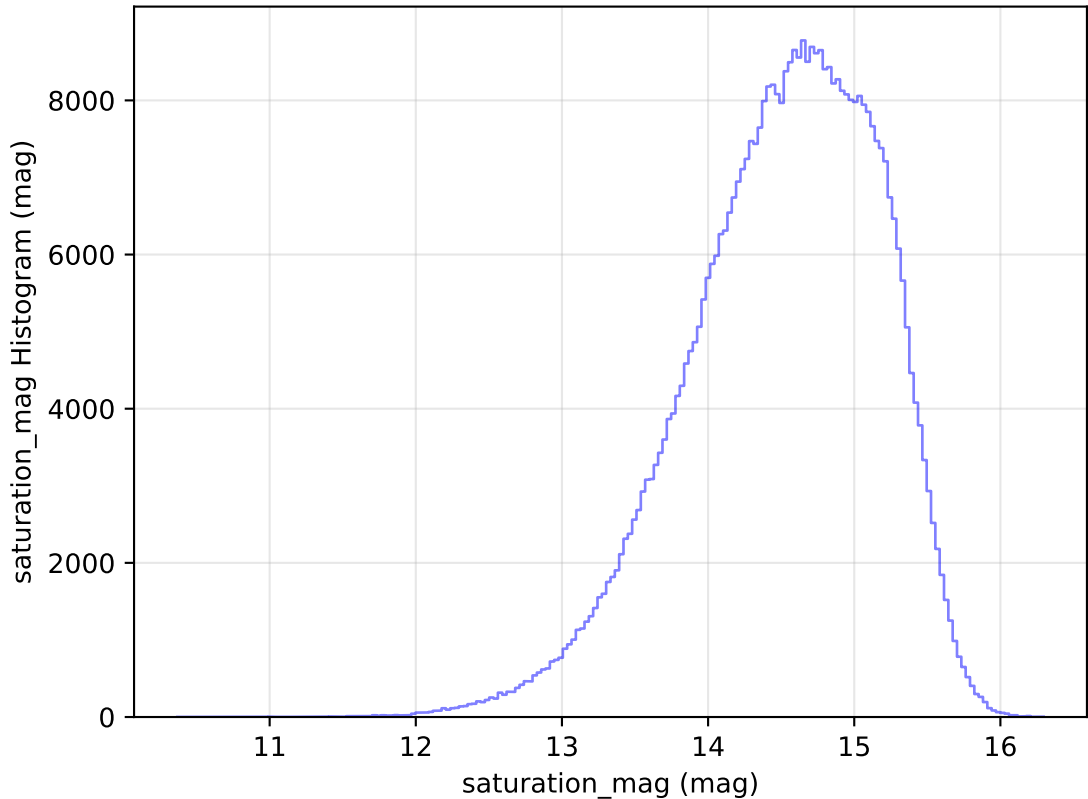
too_elab_heavy_r128_d2_griz_v3.4_10yrs WFD r band: saturation_mag Histogram
