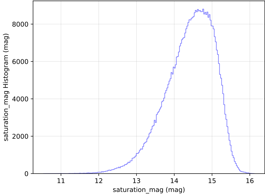
too_elab_heavy_r128_d2_griz_v3.4_10yrs WFD i band: saturation_mag Histogram
