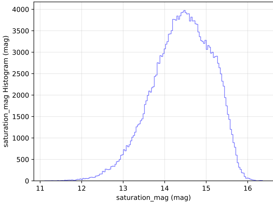
too_elab_heavy_r128_d2_griz_v3.4_10yrs WFD g band: saturation_mag Histogram
