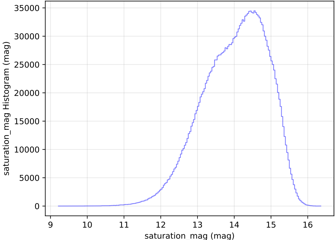
too_elab_heavy_r128_d2_griz_v3.4_10yrs WFD all bands: saturation_mag Histogram
