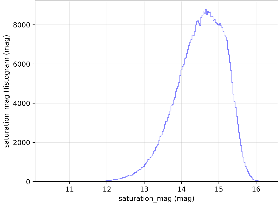
too_elab_heavy_r128_d2_griz_v3.4_10yrs All sky r band: saturation_mag Histogram
