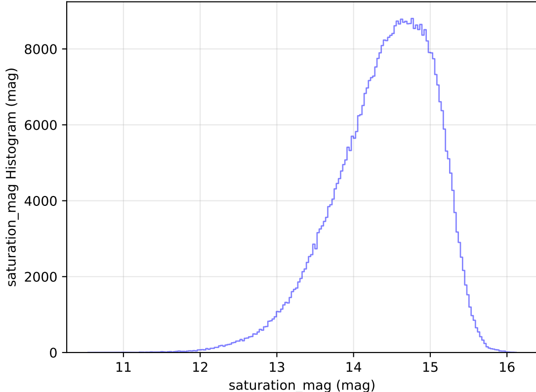
too_elab_heavy_r128_d2_griz_v3.4_10yrs All sky i band: saturation_mag Histogram
