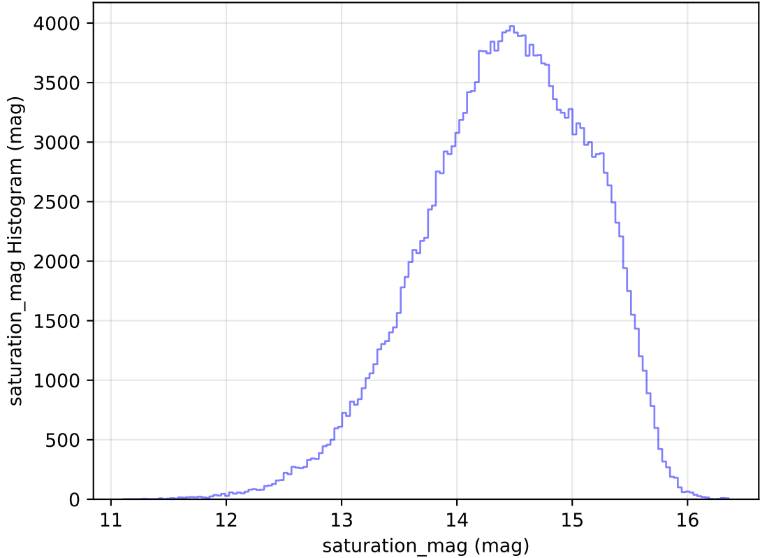
too_elab_heavy_r128_d2_griz_v3.4_10yrs All sky g band: saturation_mag Histogram
