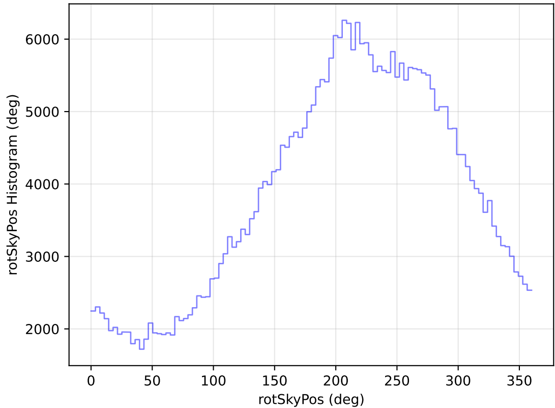
too_elab_heavy_r128_d2_griz_v3.4_10yrs WFD y band: rotSkyPos Histogram
