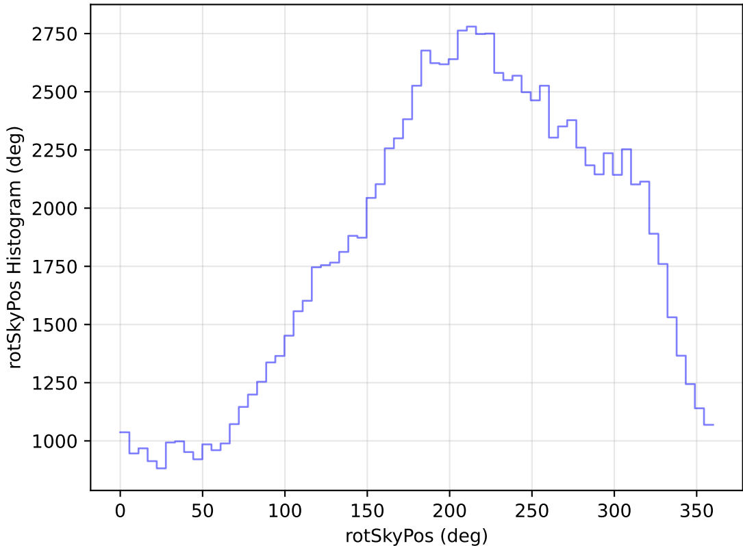
too_elab_heavy_r128_d2_griz_v3.4_10yrs WFD u band: rotSkyPos Histogram
