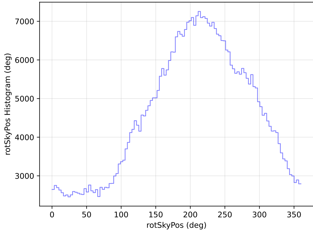
too_elab_heavy_r128_d2_griz_v3.4_10yrs WFD i band: rotSkyPos Histogram
