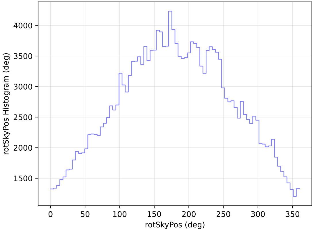
too_elab_heavy_r128_d2_griz_v3.4_10yrs WFD g band: rotSkyPos Histogram
