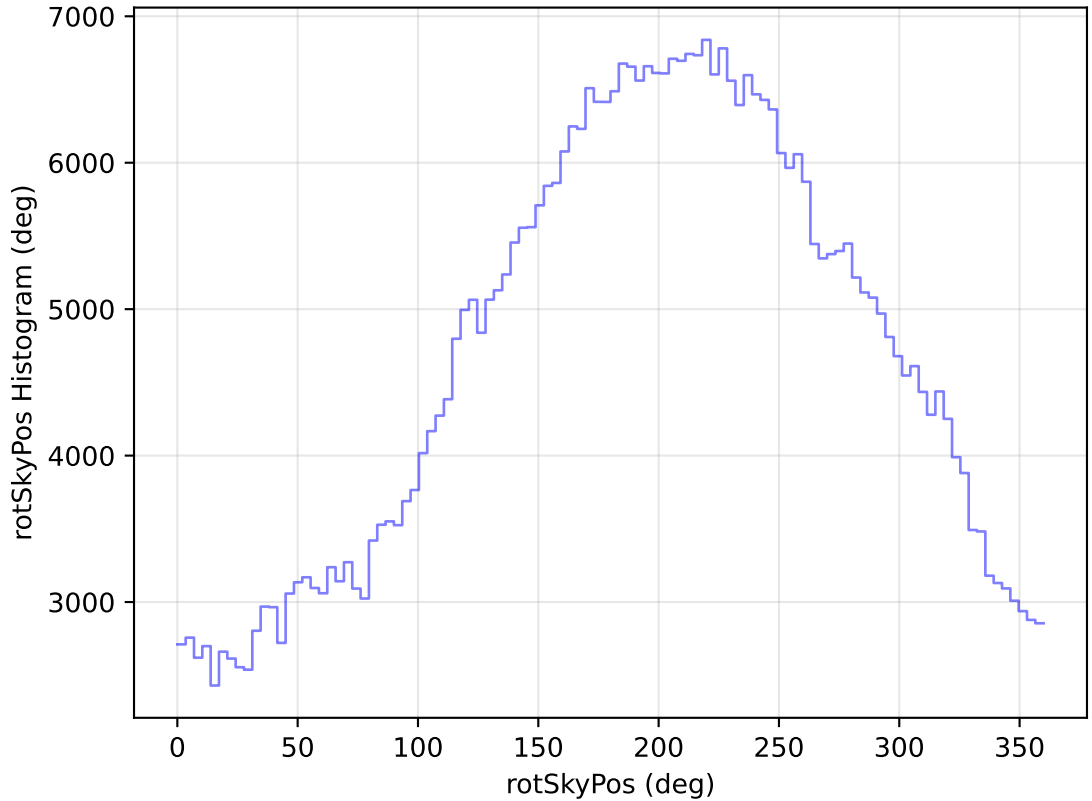
too_elab_heavy_r128_d2_griz_v3.4_10yrs All sky r band: rotSkyPos Histogram
