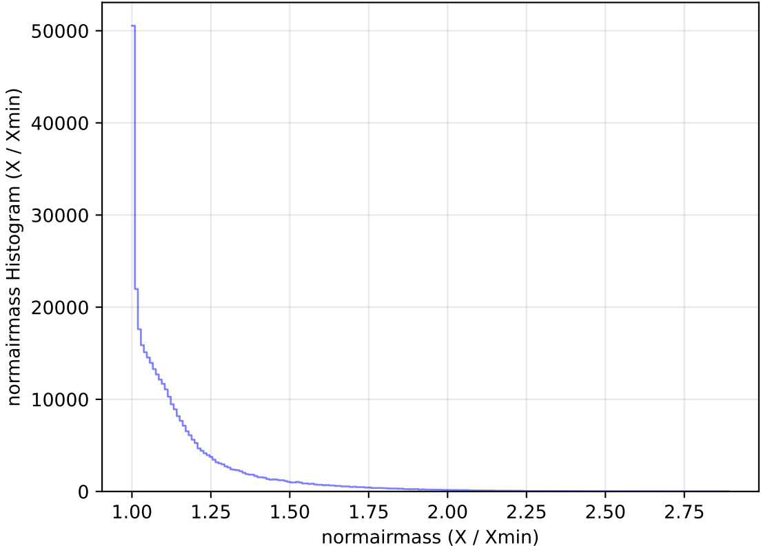
too_elab_heavy_r128_d2_griz_v3.4_10yrs WFD y band: normairmass Histogram
