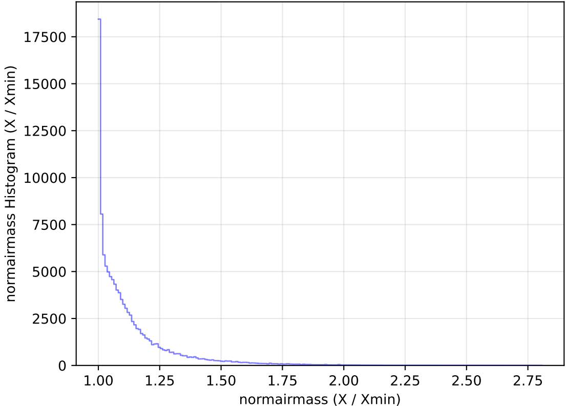
too_elab_heavy_r128_d2_griz_v3.4_10yrs WFD u band: normairmass Histogram
