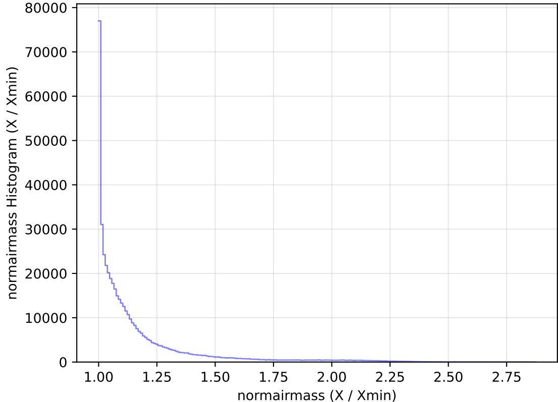
too_elab_heavy_r128_d2_griz_v3.4_10yrs WFD r band: normairmass Histogram
