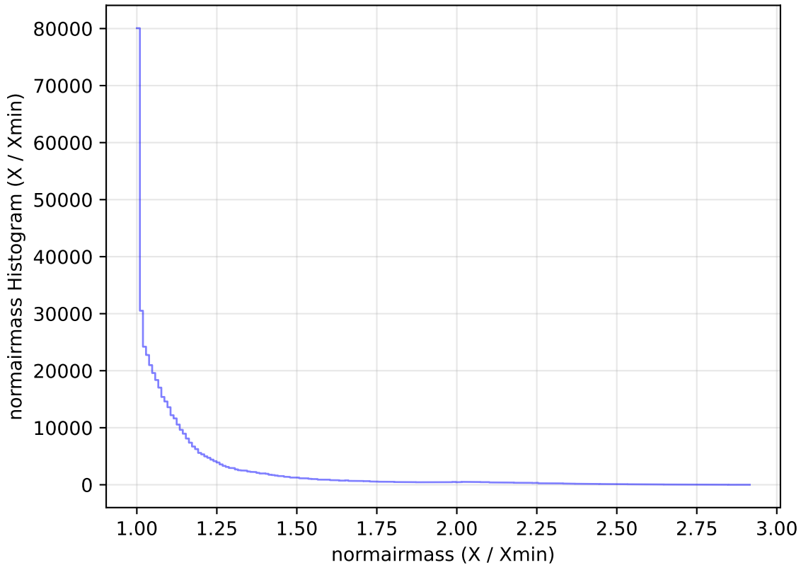
too_elab_heavy_r128_d2_griz_v3.4_10yrs WFD i band: normairmass Histogram
