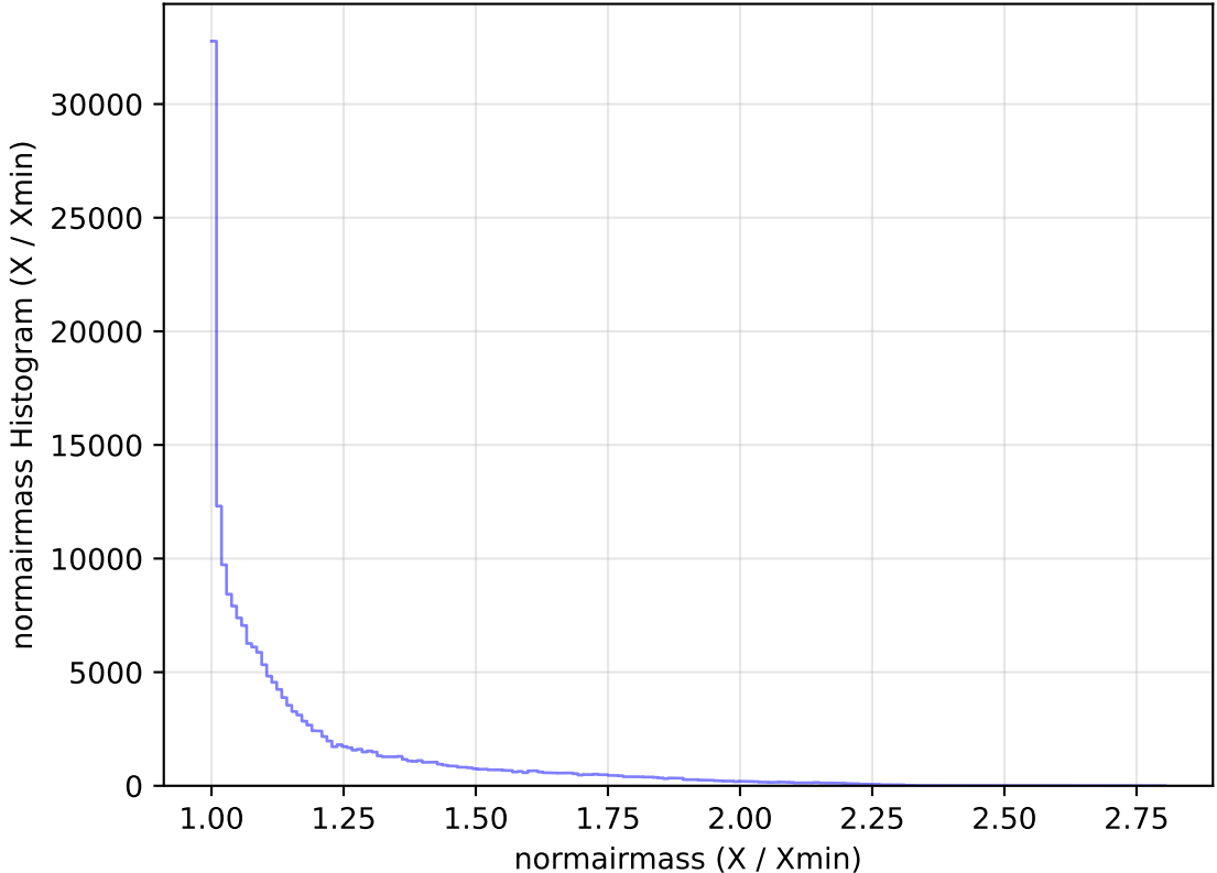
too_elab_heavy_r128_d2_griz_v3.4_10yrs WFD g band: normairmass Histogram
