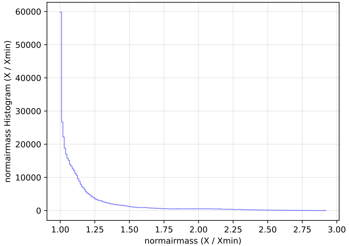
too_elab_heavy_r128_d2_griz_v3.4_10yrs All sky z band: normairmass Histogram
