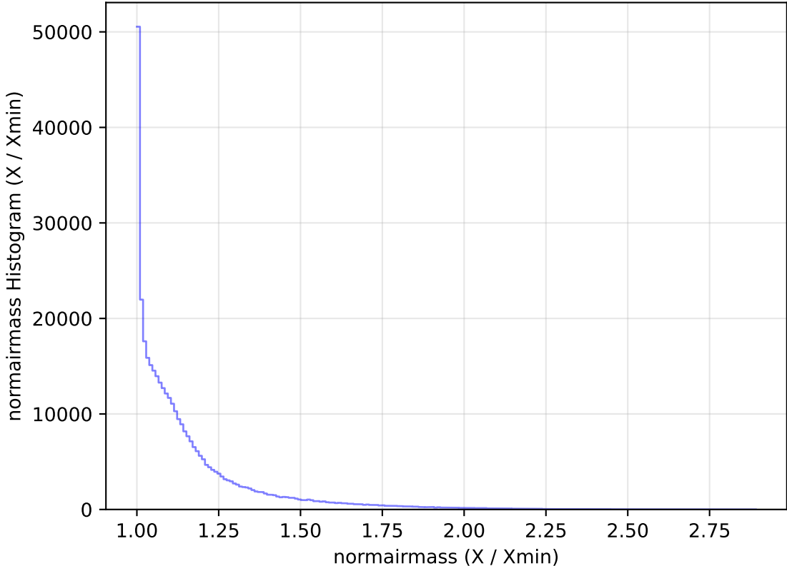
too_elab_heavy_r128_d2_griz_v3.4_10yrs All sky y band: normairmass Histogram
