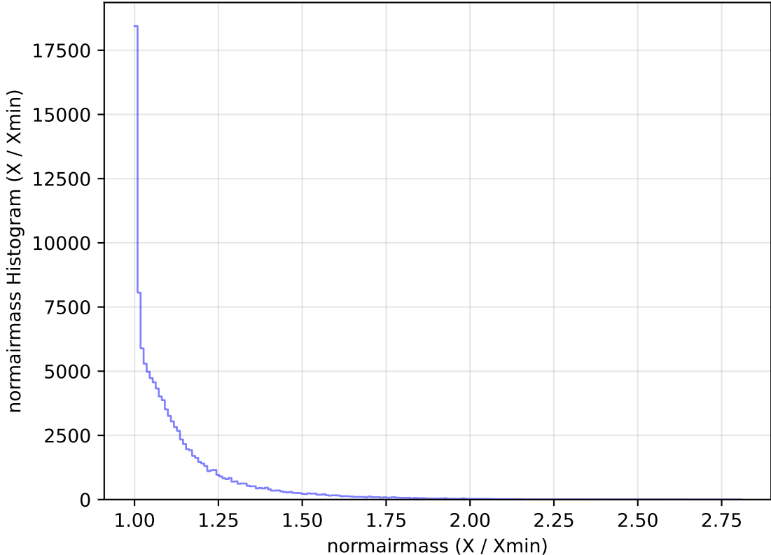
too_elab_heavy_r128_d2_griz_v3.4_10yrs All sky u band: normairmass Histogram
