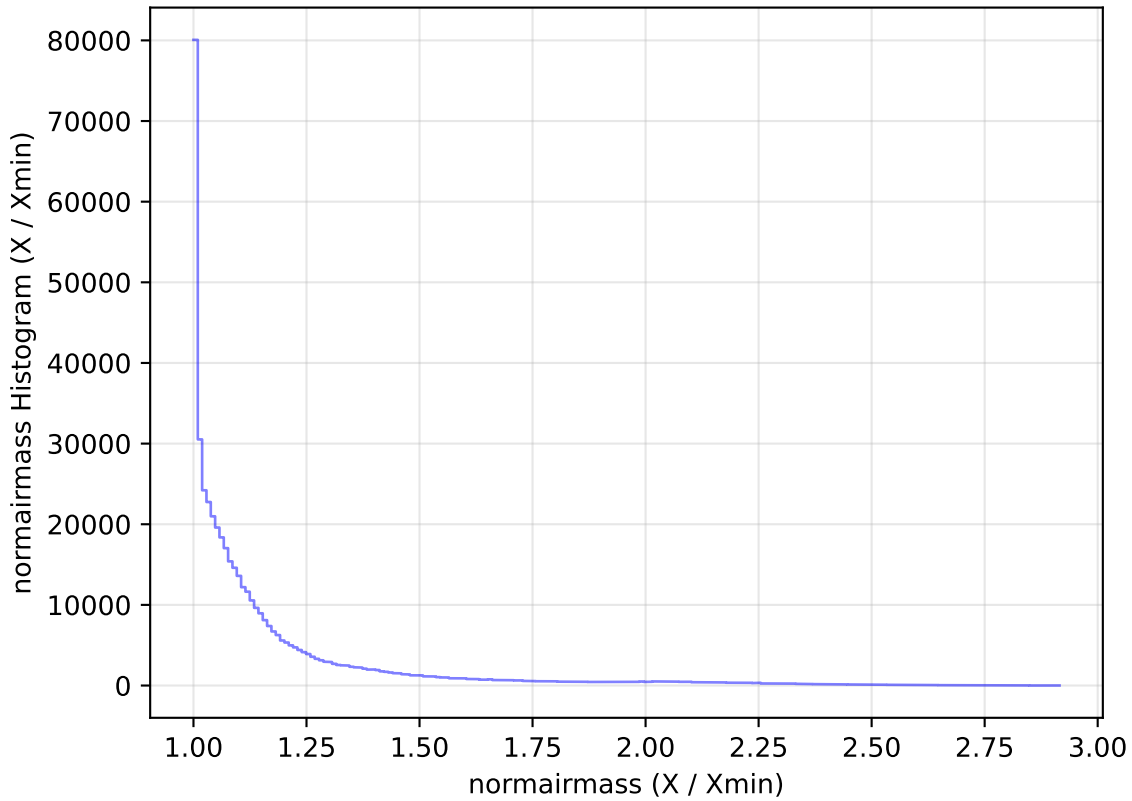
too_elab_heavy_r128_d2_griz_v3.4_10yrs All sky i band: normairmass Histogram
