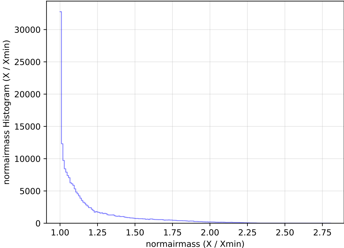
too_elab_heavy_r128_d2_griz_v3.4_10yrs All sky g band: normairmass Histogram
