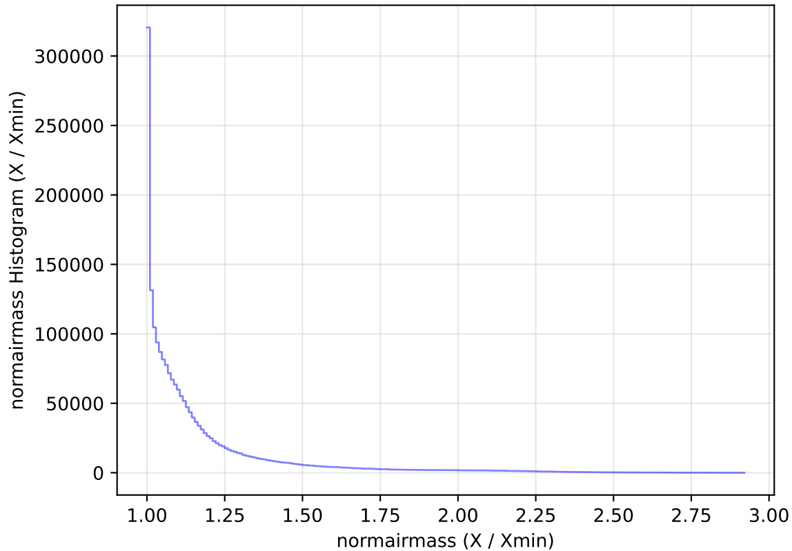
too_elab_heavy_r128_d2_griz_v3.4_10yrs All sky all bands: normairmass Histogram
