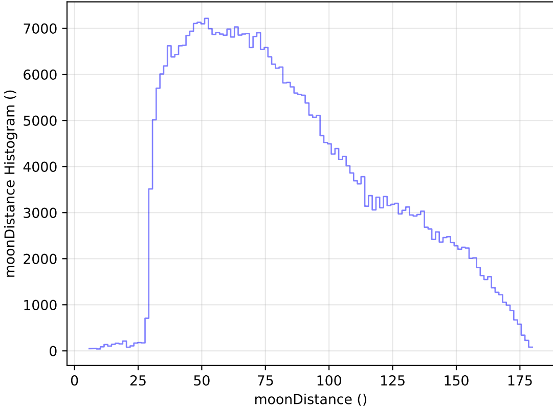
too_elab_heavy_r128_d2_griz_v3.4_10yrs WFD z band: moonDistance Histogram
